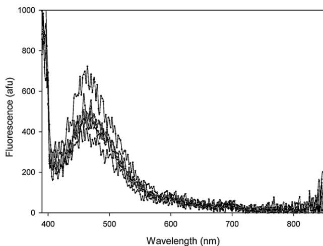
Fig. 4. Fluorescence emission spectra (400–850 nm) of whole blood from six donors at \lambda_{\text{excitation}} = 352 nm.
